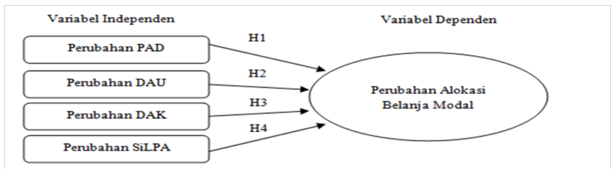
Gambar 1: Model Penelitian
